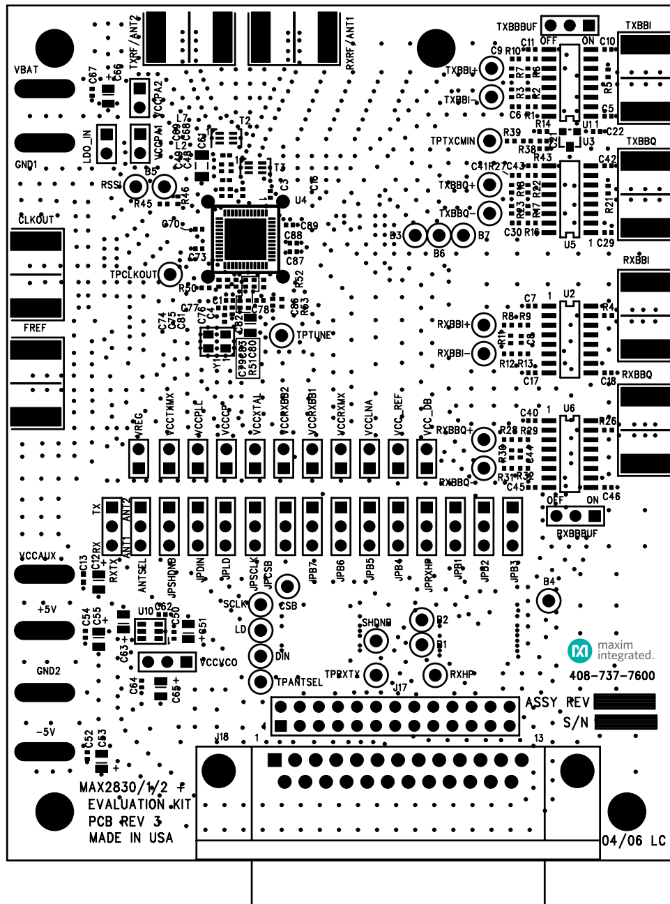
Figure 2. MAX2831 EV Kit PCB Layout—Top Silkscreen
