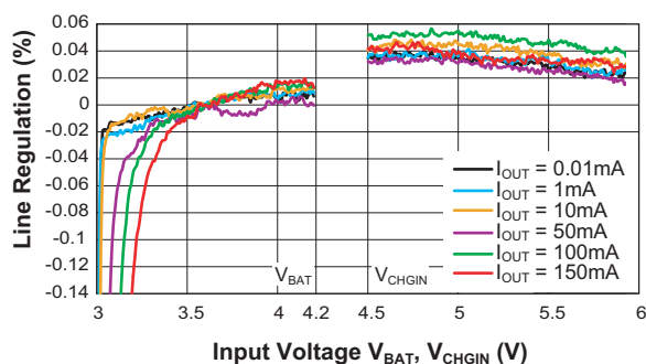
LDO4 Line Regulation vs. Battery and CHGIN Input Voltage ( V_{OUT4} = 3.0V )
