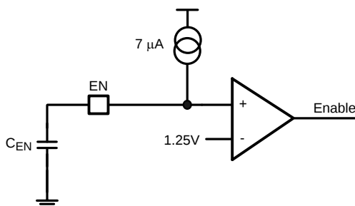
Figure 13. Cap Timing
