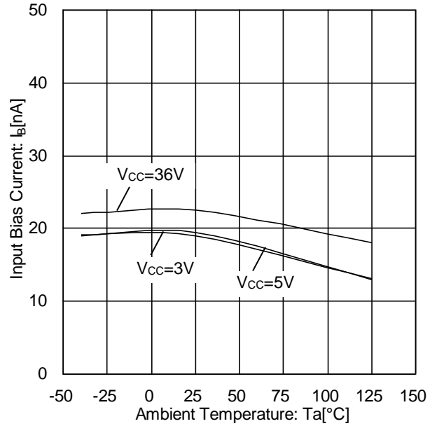
Figure 38. Input Bias Current vs Ambient Temperature ( V_{ICM}=0V , V_{OUT}=1.4V )
