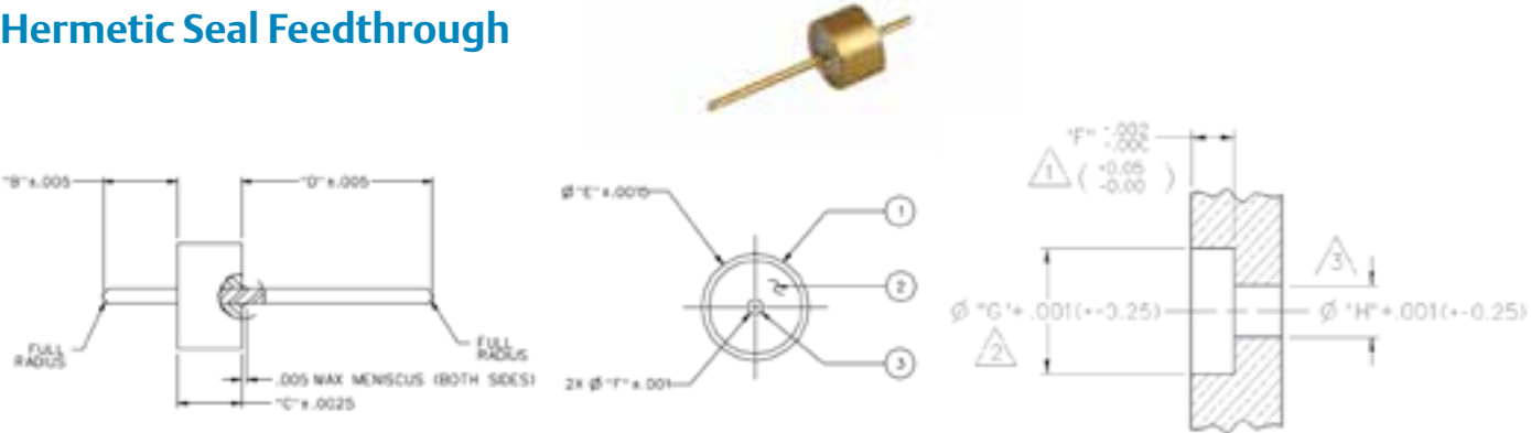
Recommended Mounting Hole Detail
