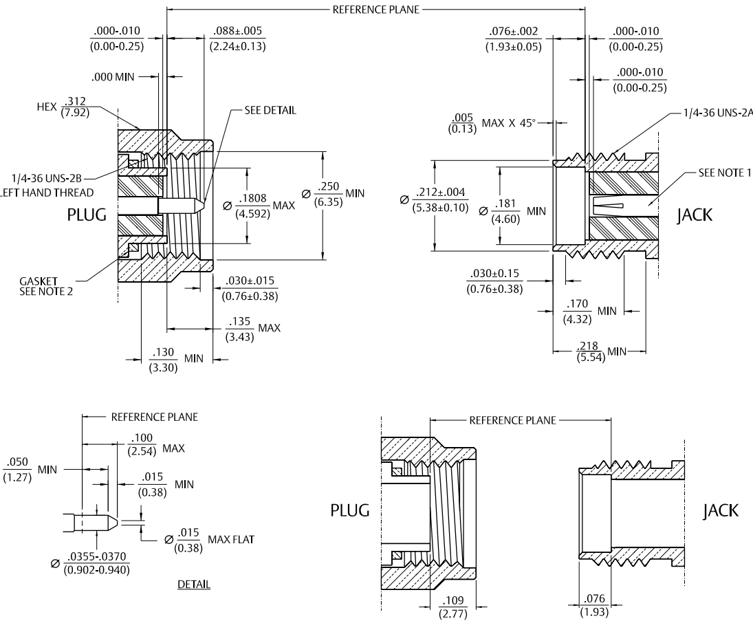
Mating Engagement for SMA Reverse Thread Series
