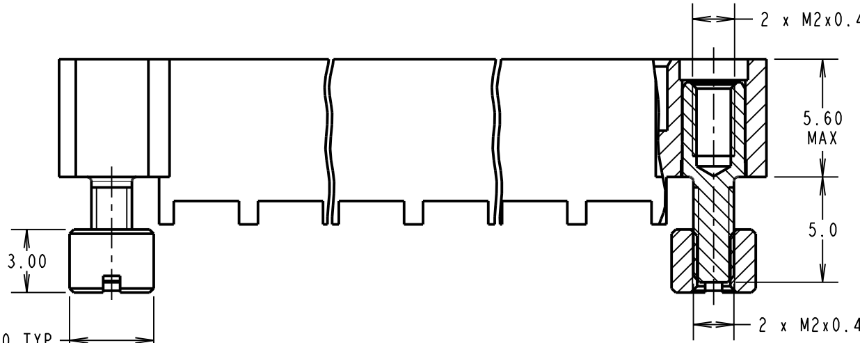
PART SECTION X-X
