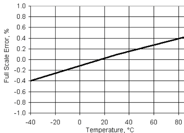
Figure 11-51. VDAC Full Scale Error vs Temperature, 1 V Mode
