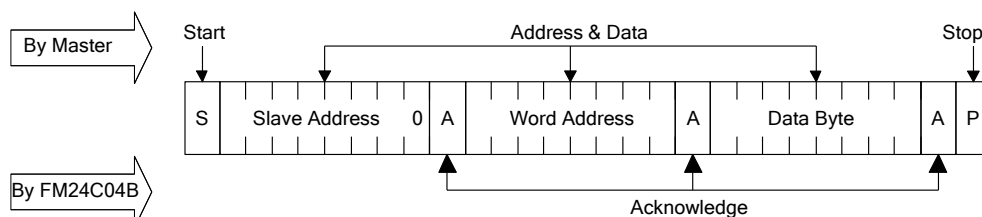
Figure 5. Byte Write
