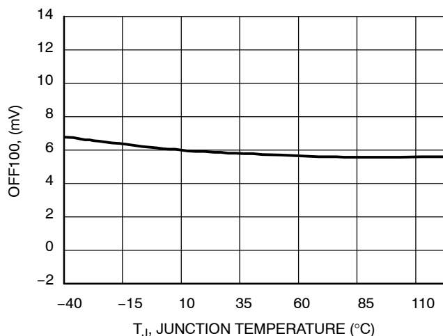
Figure 38. Current Sense Pin Voltage vs. Temperature (100 µA Being Drawn from Pin 5)
