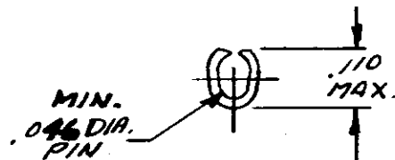
SEC. "A-A"
