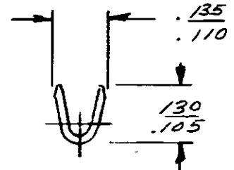
VIEW "B-B"
