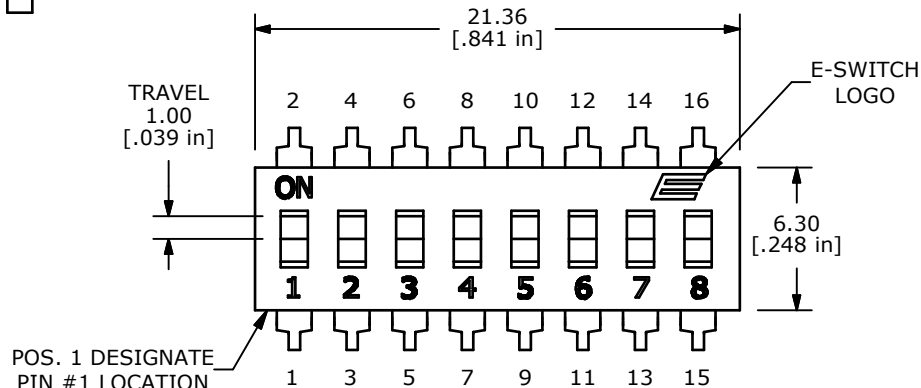
P.C.B. MOUNTING
