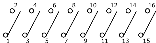
▲ CIRCUIT - 8 POSITION
