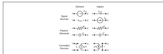
Figure 45. Individual Elements in the Current Conveyor
