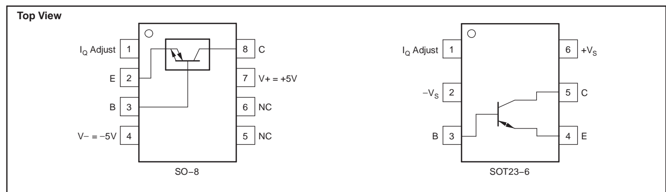
Figure 1. PIN CONFIGURATION
