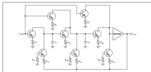
Figure 46. Universal Active Filter
