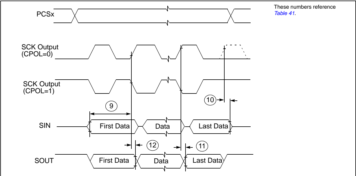
Figure 22. DSPI modified transfer format timing – master, CPHA = 1
