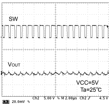
Fig.14 SW waveform I_o=10mA
