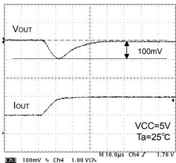
Fig. 16 Transient response I_o=1A \rightarrow 2A(10\mu s)
