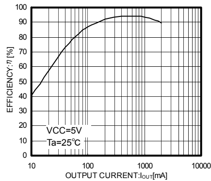
Fig.7 Efficiency
