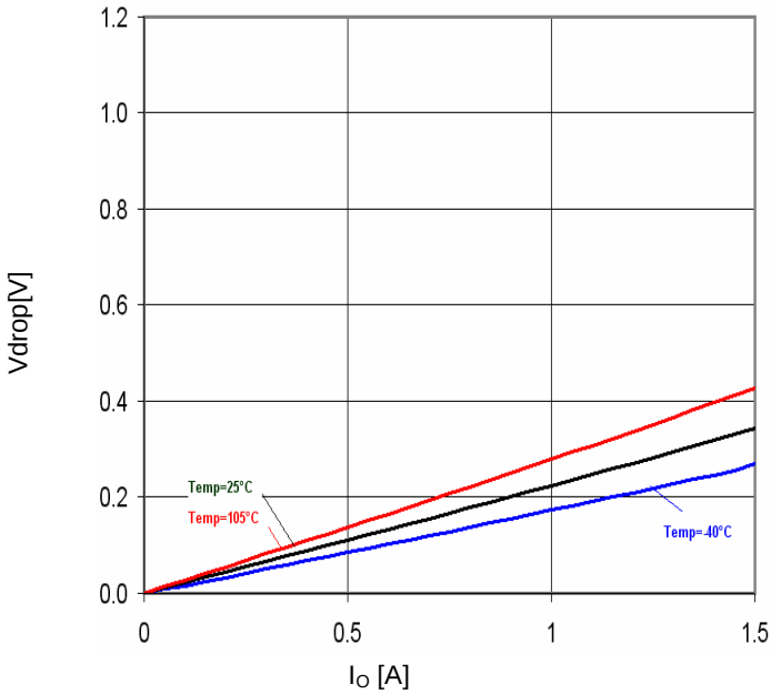
Fig.38 Minimum dropout Voltage 2 (V CC =12V, Ta=25°C)
