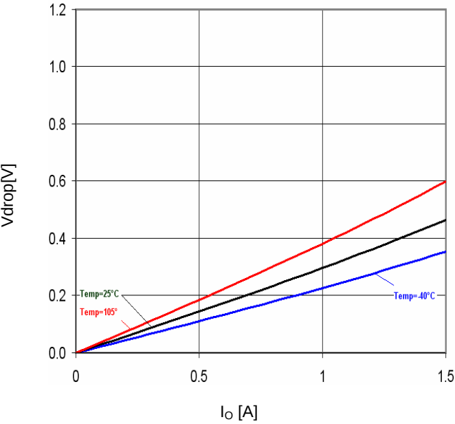
Fig.35 Minimum dropout Voltage 2 (V CC =6V, Ta=25°C)
