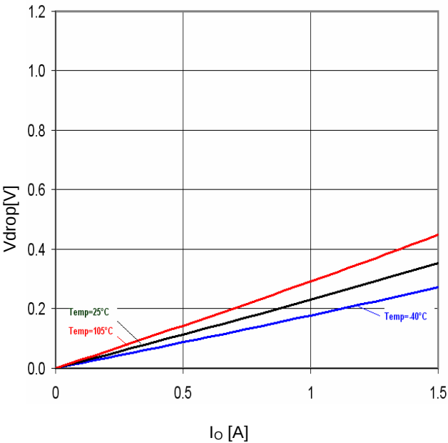
Fig.37 Minimum dropout Voltage 2 (V CC =10V, Ta=25°C)
