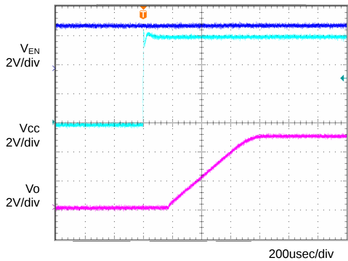
Fig.9 Input sequence 1 Co=1μF,Ta=-40°C
