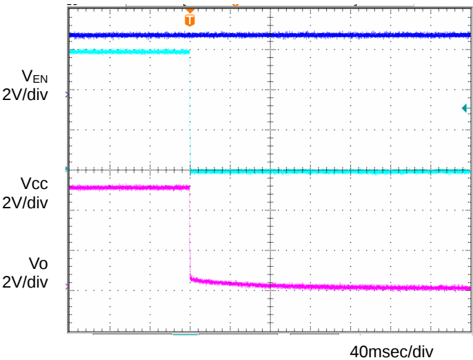
Fig.13 OFF sequence 1 Co=1μF,Ta=25°C
