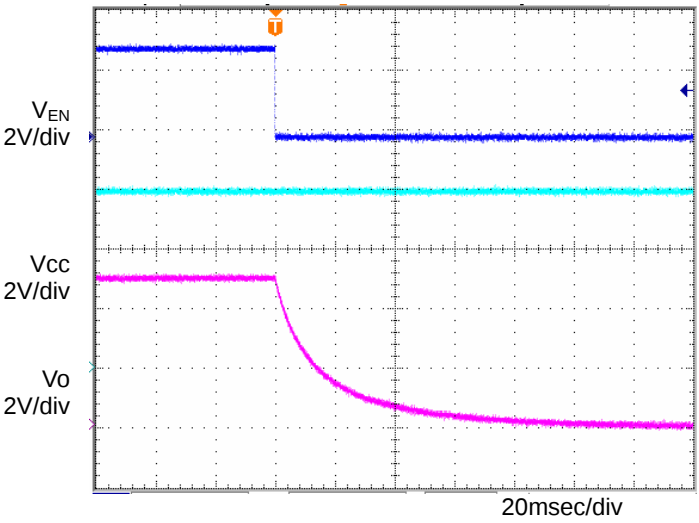
Fig.18 OFF sequence 2 C_o=1\mu F, T_a=-40^{\circ}C
