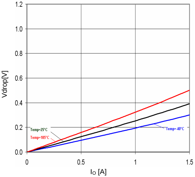
Fig.36 Minimum dropout Voltage 2 (V CC =8V, Ta=25°C)
