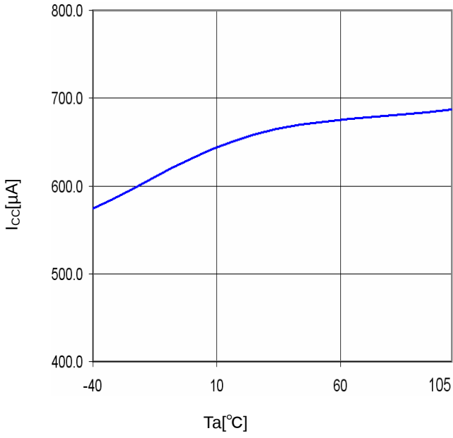
Fig.22 T_a - I_{cc}
