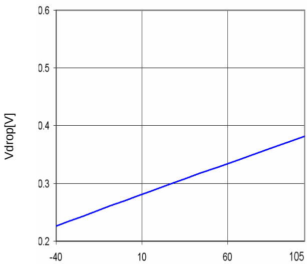
Fig.30 Minimum dropout Voltage1 ( V_{cc}=6\text{V} , I_o=1.0\text{A} )
