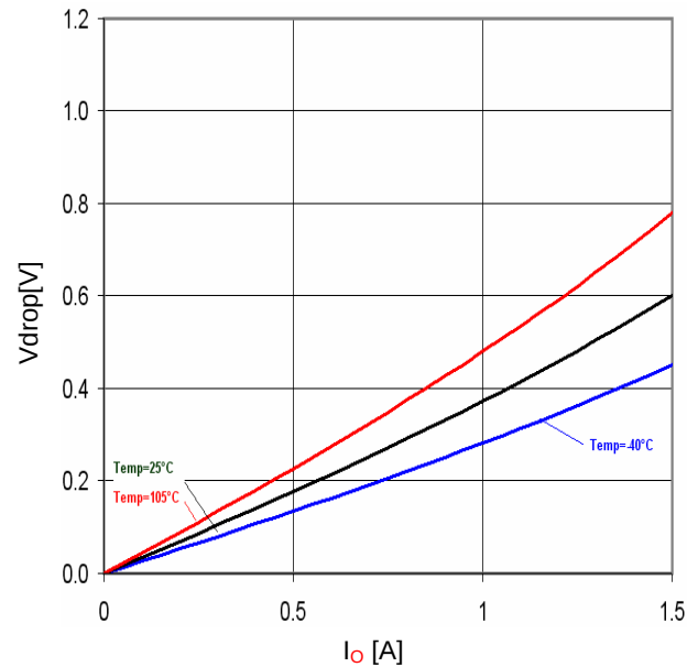
Fig.34 Minimum dropout Voltage 2 ( V_{CC}=4.5 V、 T_a=25^{\circ} C)
