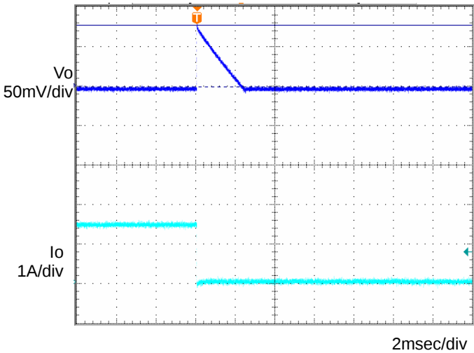
Fig.8 Transient Response (1.0→0A) Co=1μF,Ta=105°C
