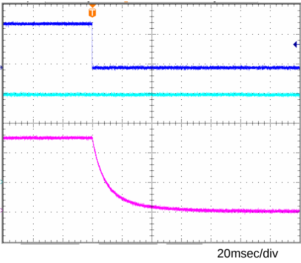
Fig.20 OFF sequence 2 C_o = 1\mu\text{F} , T_a = 105^\circ\text{C}
