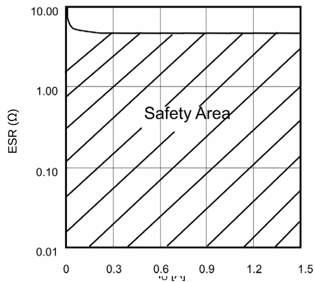
Fig.31 Operation Safety area
