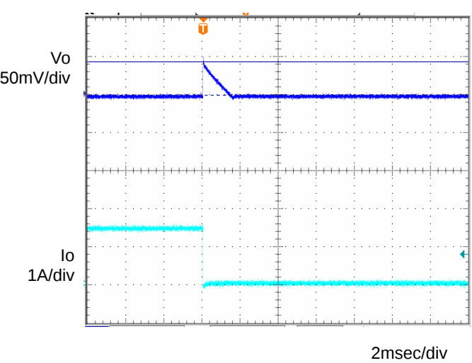
Fig.6 Transient Response (1.0→0A) Co=1μF, Ta=-40°C
