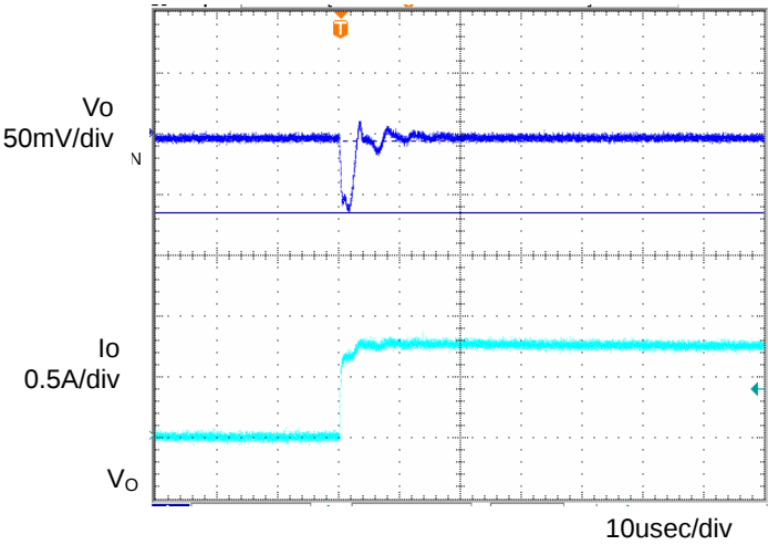
Fig.5 Transient Response (0 \rightarrow 1.0A) Co=1 \mu F, Ta=-40°C
