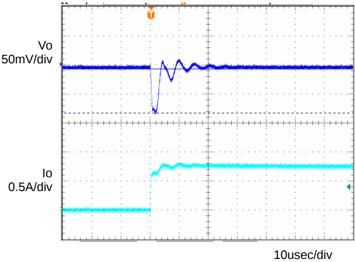
Fig.5 Transient Response (0 \rightarrow 1.0A) Co=1 \mu F, Ta=105°C
