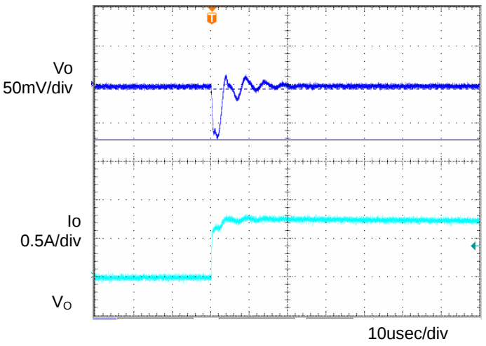
Fig.6 Transient Response (1.0 \rightarrow 0A) Co=1 \mu F, Ta=25°C
