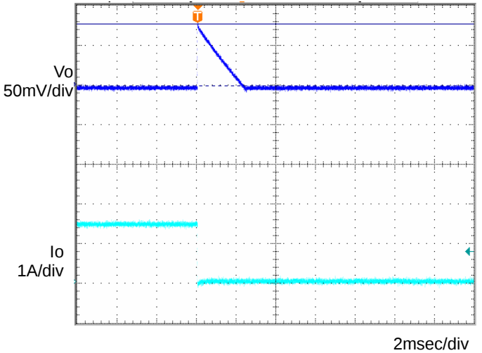
Fig.8 Transient Response (1.0→0A) C_o=1\mu\text{F} , T_a=105^\circ\text{C}
