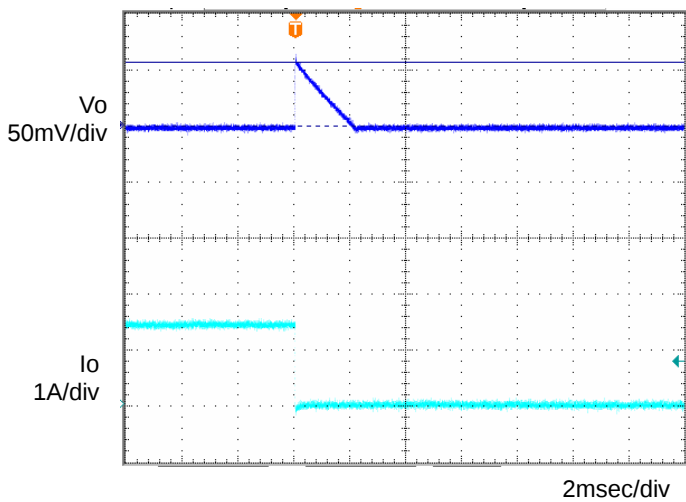
Fig.7 Transient Response (1.0→0A) C_o=1\mu\text{F} , T_a=25^\circ\text{C}
