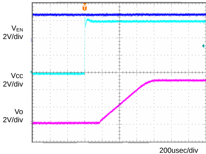
Fig.9 Input sequence 1 C_o=1\mu\text{F} , T_a=-40^\circ\text{C}
