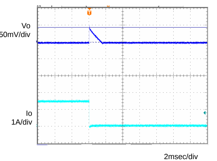
Fig.6 Transient Response (1.0→0A) Co=1μF, Ta=-40°C
