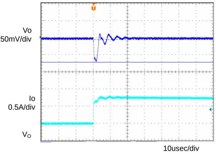
Fig.6 Transient Response (1.0→0A) Co=1μF, Ta=25°C
