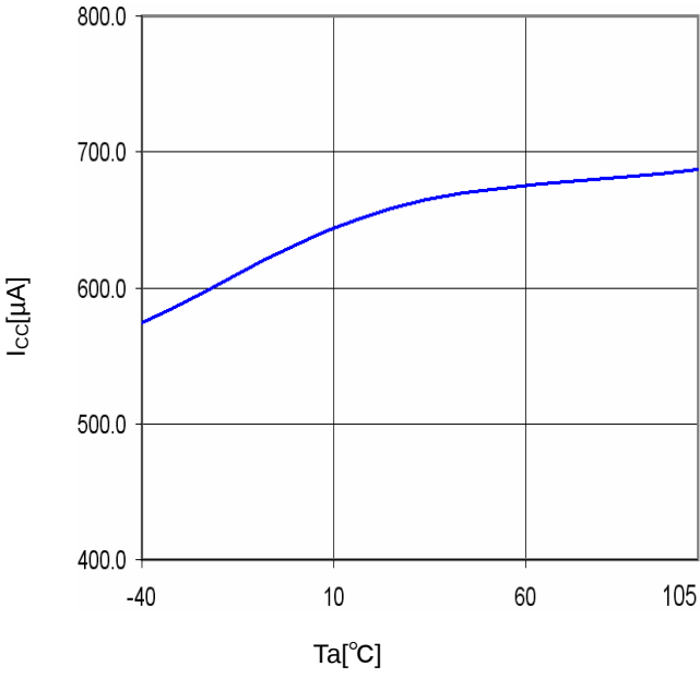
Fig.22 T_a - I_{cc}
