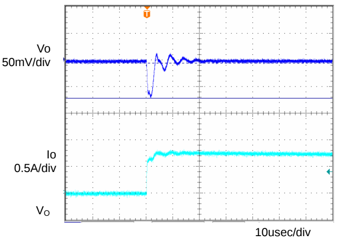
Fig.6 Transient Response (1.0 \rightarrow 0A) Co=1 \mu F, Ta=25 ^{\circ} C
