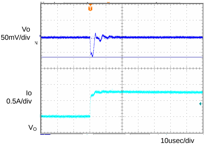
Fig.5 Transient Response (0 \rightarrow 1.0A) Co=1 \mu F, Ta=-40 ^{\circ} C
