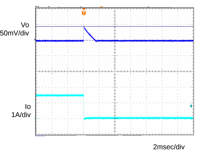
Fig.6 Transient Response (1.0 \rightarrow 0A) Co=1 \mu F, Ta=-40 ^{\circ} C
