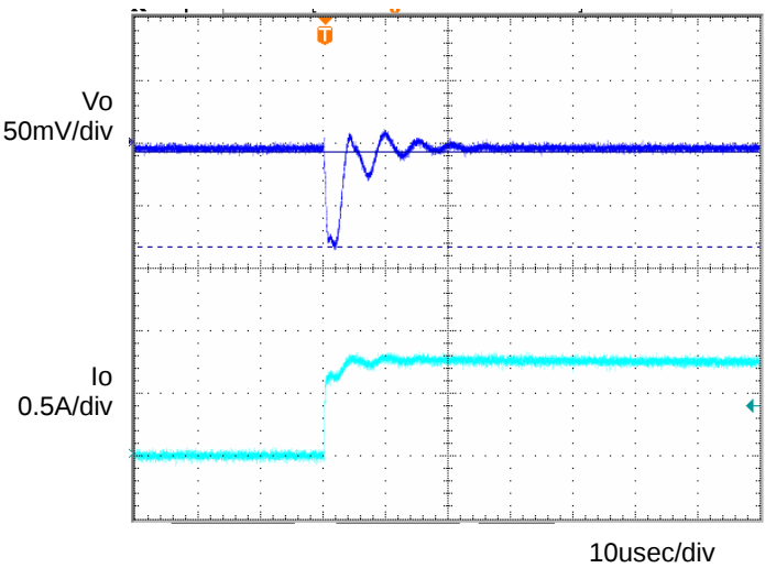
Fig.5 Transient Response (0 \rightarrow 1.0A) Co=1 \mu F, Ta=105 ^{\circ} C
