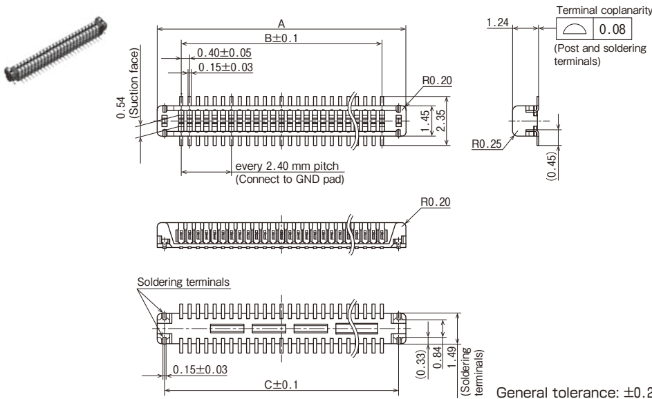
Dimension table
