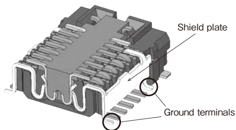
<Ground terminal cross-section diagram>
