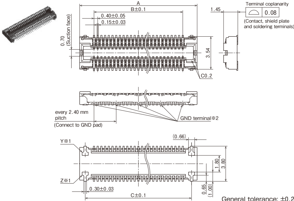
Dimension table
