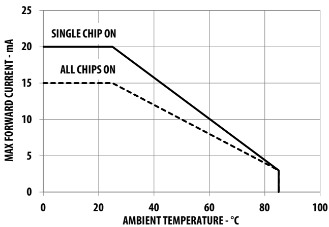
Figure 6: Derating Curve
