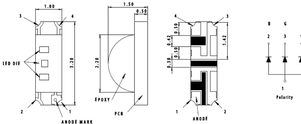
Figure 1: Package Dimensions
