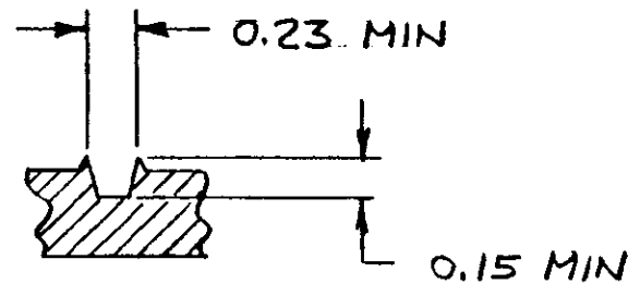
SECTION A-A TYP. SERRATION
