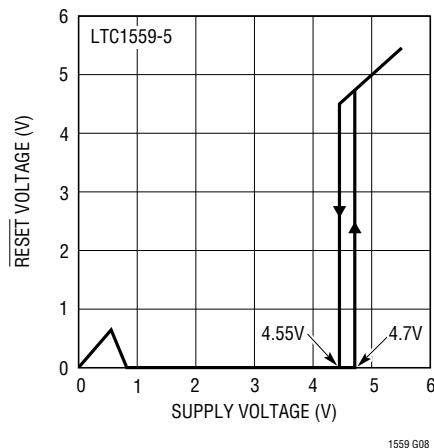
RESET Output Voltage vs Supply Voltage
