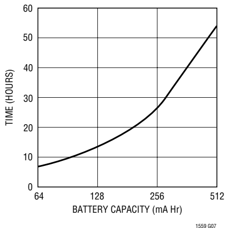
Fast Recharge Time (Assume NiCd Battery Fully Exhausted)
