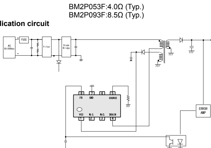
Figure 1. Application circuit
