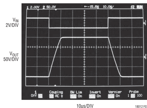
Figure 7. Large-Signal Time Domain Response of the Amplifier
