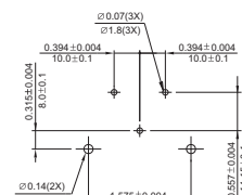
MOUNTING DIMENSIONS OF PC BOARD
