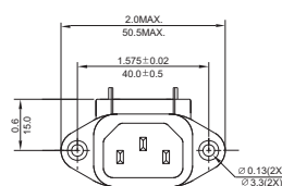
SUGGESTED MOUNTING CUTOUT (MOUNTING DIMENSIONS OF SOCKET)
