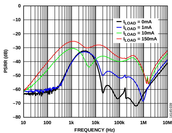
Figure 40. Power Supply Rejection Ratio (PSRR) vs. Frequency
