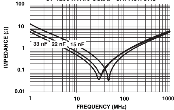
IMPEDANCE VS. FREQUENCY OF 1206 HV Arc Guard® CAPACITORS
