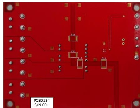
Figure 2. BD7F200HFN-EVK-001 Evaluation Board
