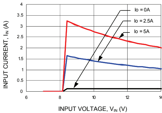
Figure 7. Input voltage vs. Input Current (V out = 5.0Vdc).
