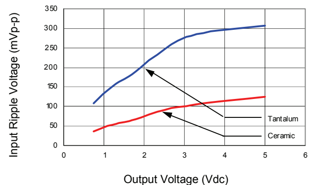
Figure 26. Input ripple voltage for various output with 2x47 µF tantalum capacitors and with 2x22 µF ceramic capacitors at the input (100% of I_{O,max} ).
