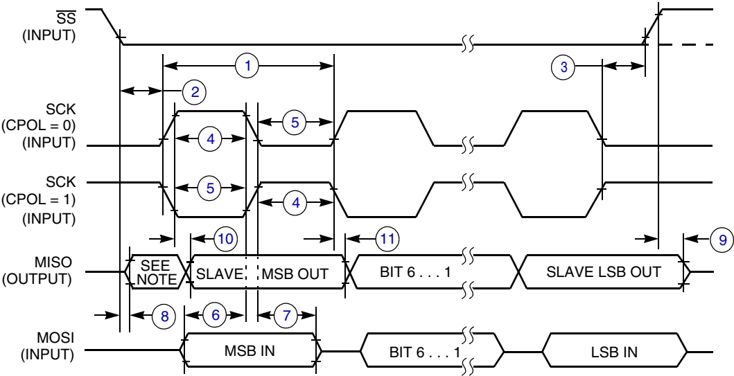
NOTE: 1. Not defined but normally LSB of character just received Figure A-13. SPI Slave Timing (CPHA = 1)
