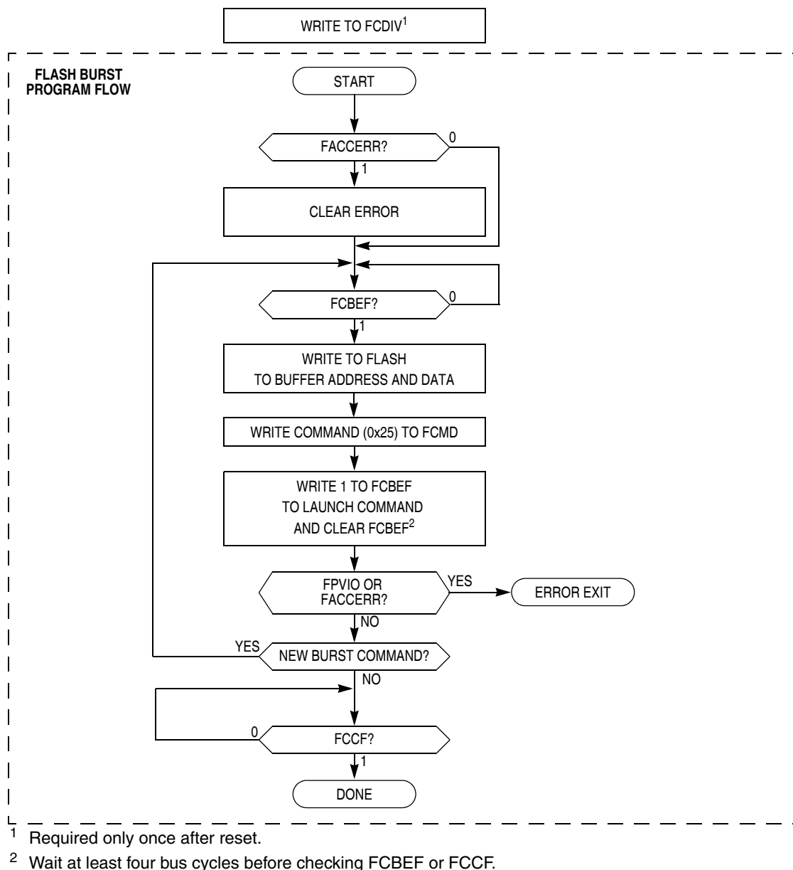
Figure 4-3. Flash Burst Program Flowchart
