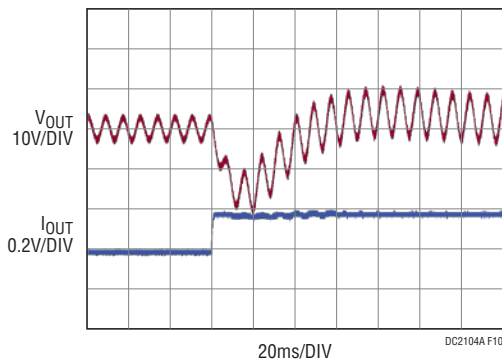
Figure 10. V_{IN} = 115VAC , Half Load to Full Load Transient
