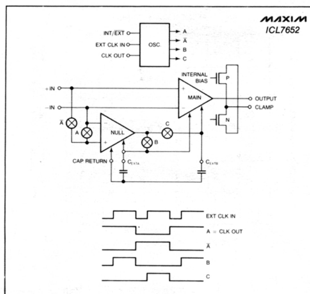
Figure 2. Maxim ICL7652 Block Diagram
