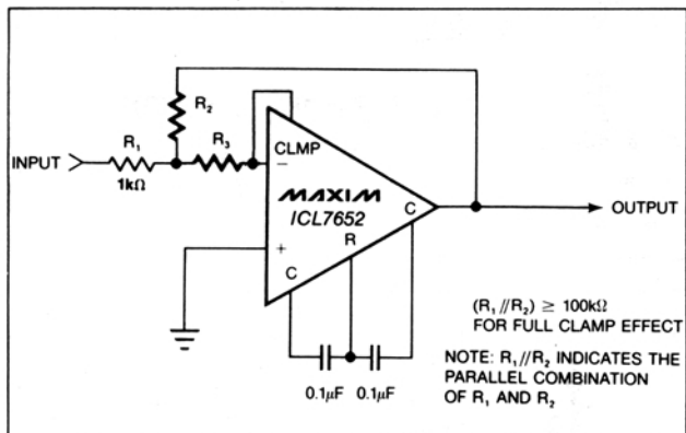
Figure 5. Inverting Amplifier with Optional Clamp
