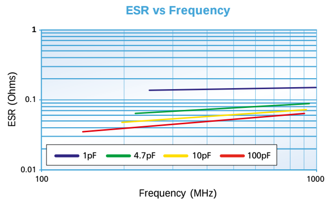
Typical performance data - chip size 1111 High Q
