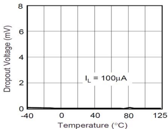
Figure 19. Dropout Voltage
