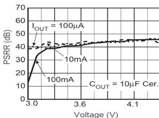
Figure 10. PSRR vs. Voltage Drop
