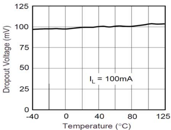
Figure 20. Dropout Voltage
