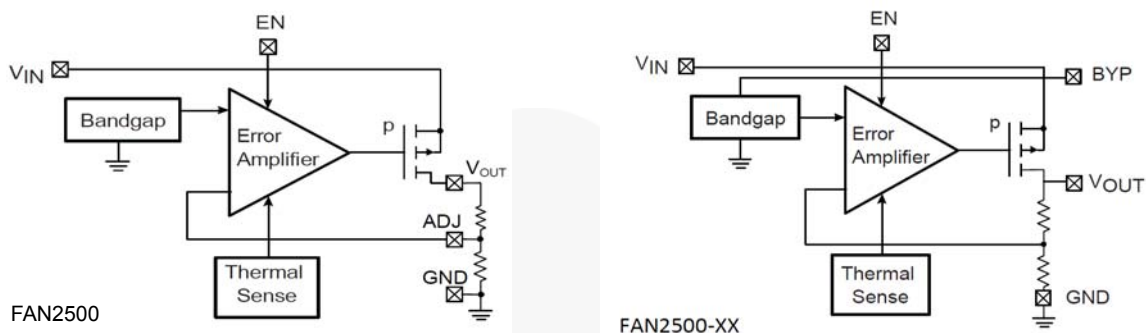
Figure 1. Block Diagram
