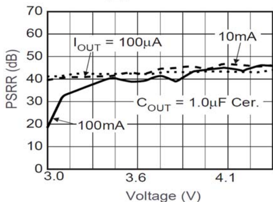
Figure 9. PSRR vs. Voltage Drop
