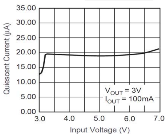
Figure 14. Ground Pin Current
