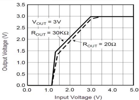
Figure 18. Dropout Characteristics
