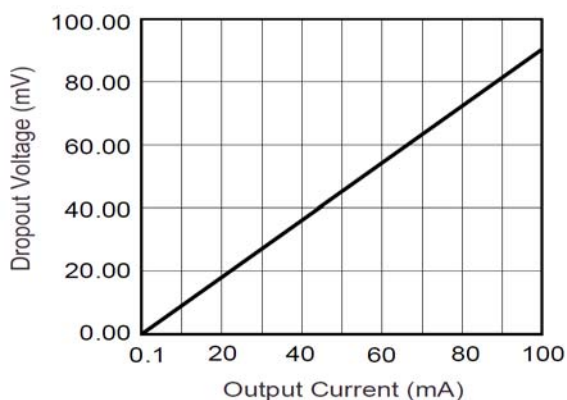
Figure 17. Dropout Voltage
