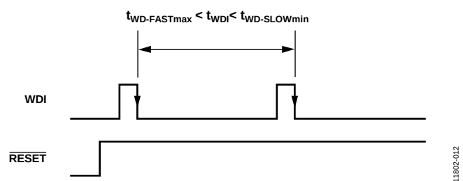
Figure 23. Normal Watchdog Operation
