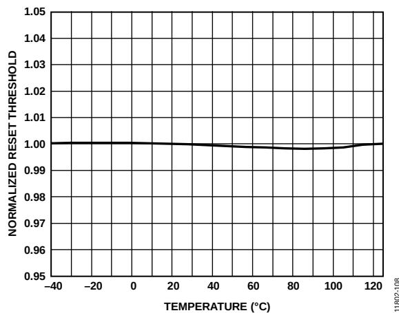
Figure 6. Normalized Reset Threshold vs. Temperature
