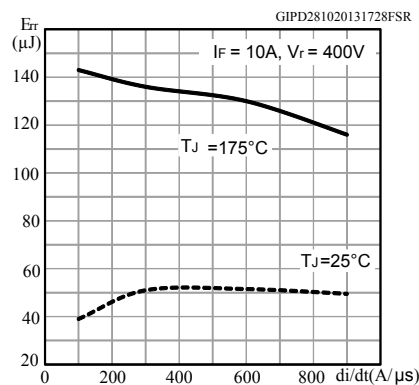
Figure 29. Reverse recovery energy vs diode current slope
