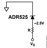
Figure 20. Negative Precision Reference Configuration
