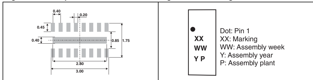
Figure 9. Footprint
