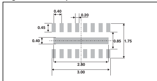
Figure 9. Footprint
