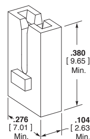
Cavity Specification 1601425
