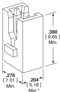
Cavity Specification 1601421
