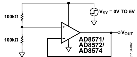
Figure 62. AD857x Test Circuit for Power-Up Time
