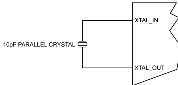
Figure 6. Crystal Input Interface
