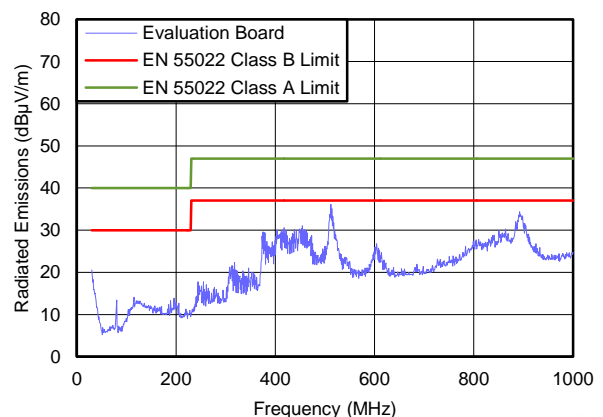
Radiated EMI (CISPR22) V_{IN} = 5.0V, V_{OUT} = 1.8V, I_{OUT} = 1A
