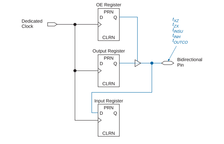
Figure 38. External Timing in Cyclone Devices
