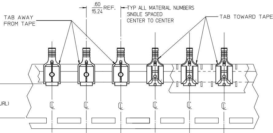
PARTS ON TAPE (SCALE 2:1) D
