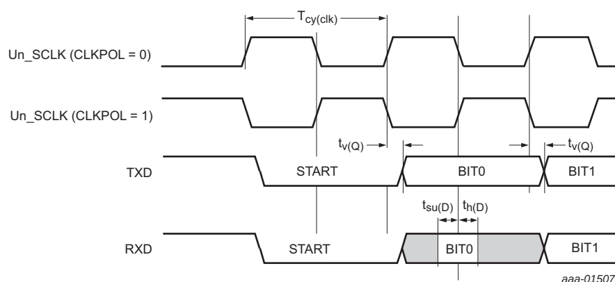
Fig 36. USART timing
