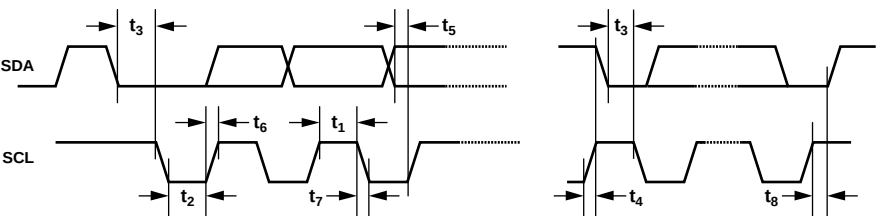
Figure 3. I²C Timing
