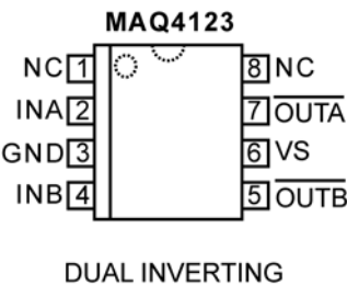
DUAL INVERTING
