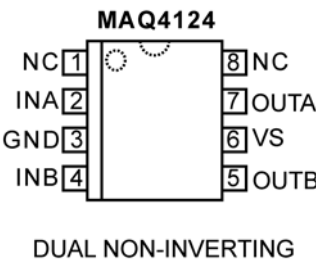
DUAL NON-INVERTING
